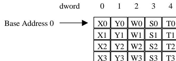
Figure: AOS Vertex Data Storage
